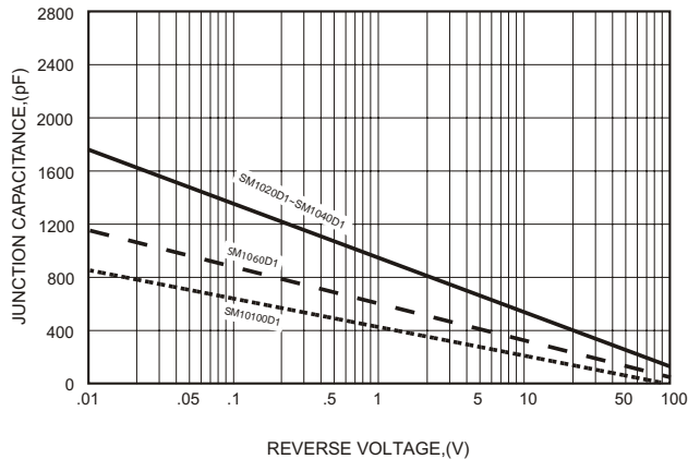
FIG.4-TYPICAL JUNCTION CAPACITANCE
