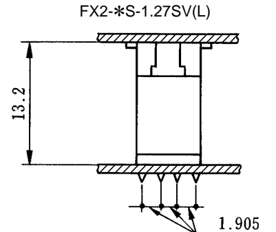
FX2C(A)1-*P-1.27DSA(L)
