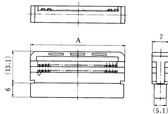
Combination View
