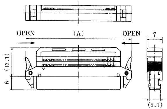
Combination View
