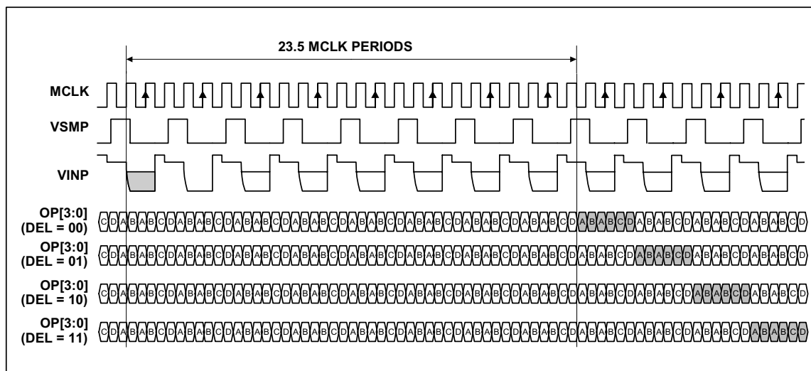
Figure 16 Mode 2 Operation
