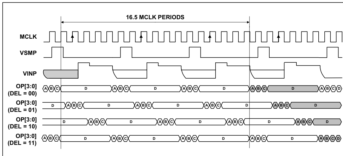
Figure 15 Mode 1 Operation
