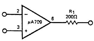
OUTPUT SHORT-CIRCUIT PROTECTION
