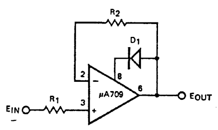
LATCH-UP PROTECTION
