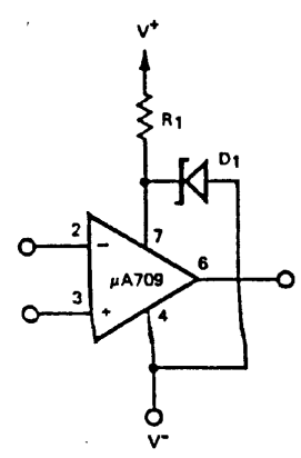
SUPPLY OVERVOLTAGE-PROTECTION
