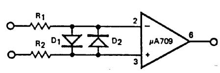
INPUT BREAKDOWN-PROTECTION
