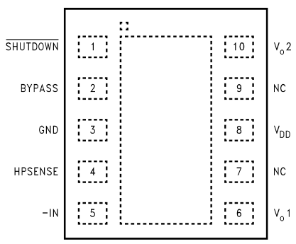
Top View Order Number LM4892LD See NS Package Number LDA10B
