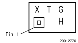
Top View X - Date Code T - Die Traceability G - Boomer Family H - LM4892IBP
