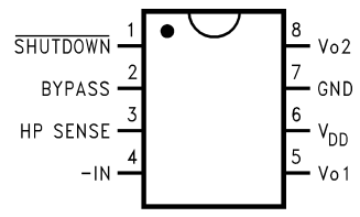
Top View Order Number LM4892M See NS Package Number M08A
