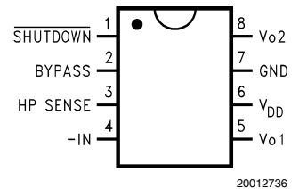
Top View Order Number LM4892MM See NS Package Number MUA08A
