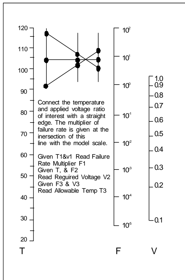
Fig.8 Reliability Nomograph
