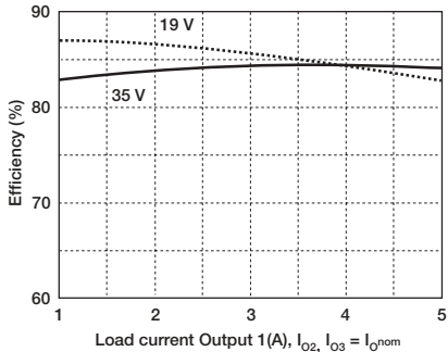
Efficiency (typ)
