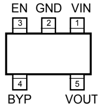
MIC5319-x.xBD5/YD5 TSOT-23-5 (D5) (Top View)
