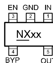
MIC5256-x.xYD5 5-Pin Thin SOT23
