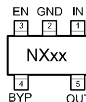
MIC5256-x.xBD5 5-Pin Thin SOT23
