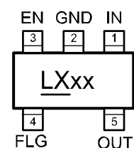
MIC5256-x.xYM5 5-Pin SOT23
