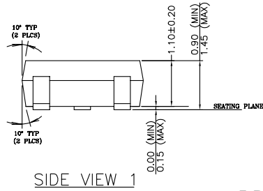
SIDE VIEW 1
