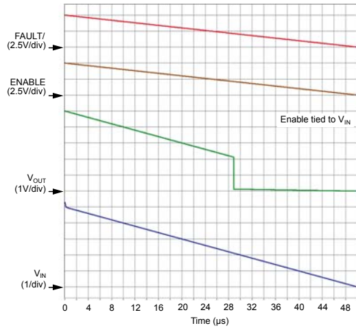
UVLO Decreasing
