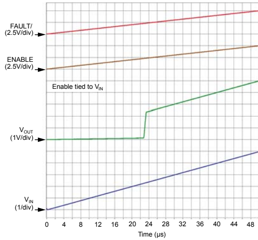
UVLO Increasing
