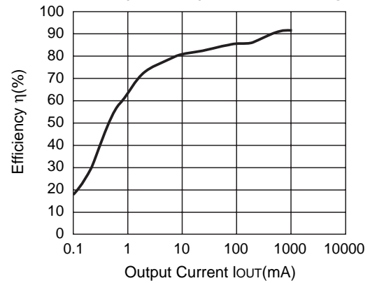
R1224N332E (V IN =7.0V) CDRH127-10μH
