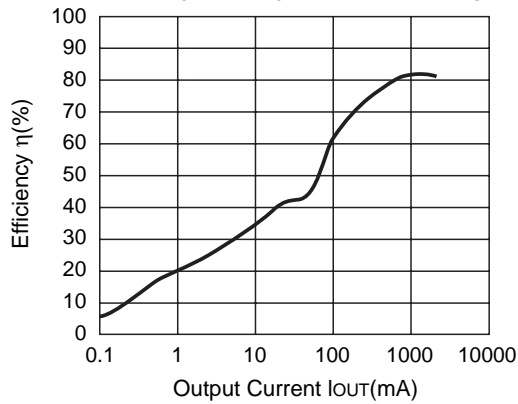
R1224N182M (V IN =12V) CDRH127-27μH
