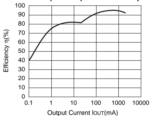
R1224N332L ( V_{IN}=4.8V ) CDRH127-27 \mu H
