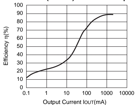
R1224N332M ( V_{IN}=12V ) CDRH127-27 \mu H
