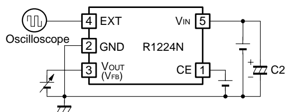
Output Delay Time for Protection Circuit
