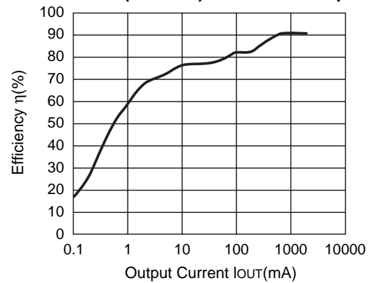
R1224N332F (V IN =7.0V) CDRH127-10μH
