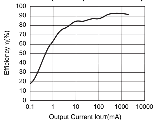
R1224N332L ( V_{IN}=7.0V ) CDRH127-27 \mu H
