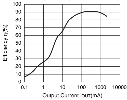
R1224N182M (V IN =3.3V) CDRH127-27μH
