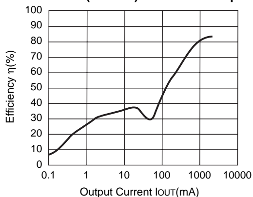
R1224N332H ( V_{IN}=15V ) CDRH127-10 \mu H
