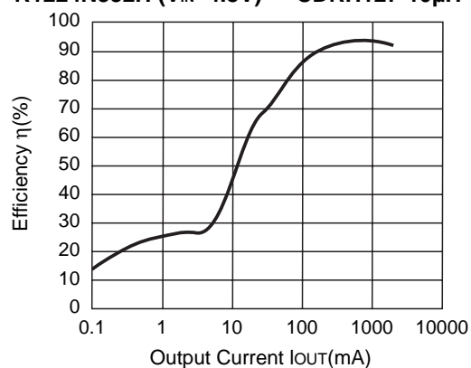
R1224N332H ( V_{IN}=4.8V ) CDRH127-10 \mu H
