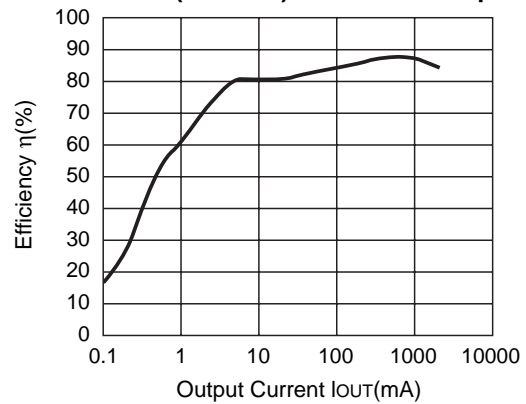
R1224N182L (V IN =5.0V) CDRH127-27μH
