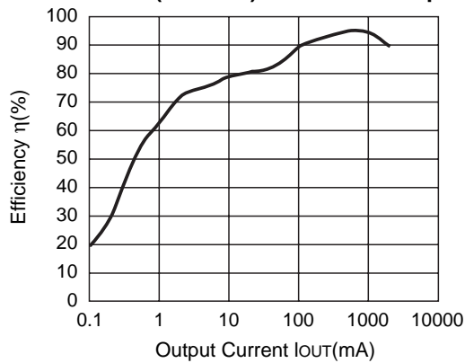
R1224N332E (V IN =4.8V) CDRH127-10μH
