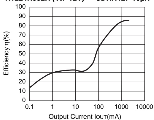
R1224N332H ( V_{IN}=12V ) CDRH127-10 \mu H
