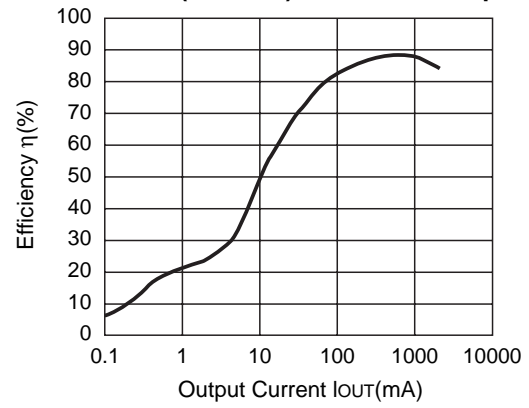
R1224N182M (V IN =5.0V) CDRH127-27μH
