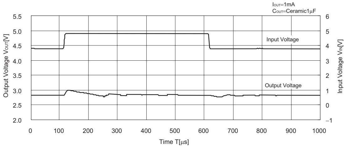
R1180x281x
