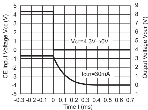
R1161x33xD
