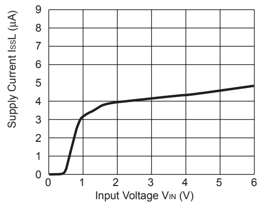
R1161x15xx (ECO=L)
