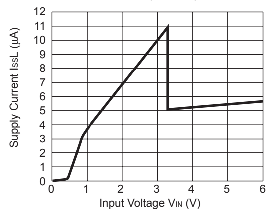
R1161x33xx (ECO=L)
