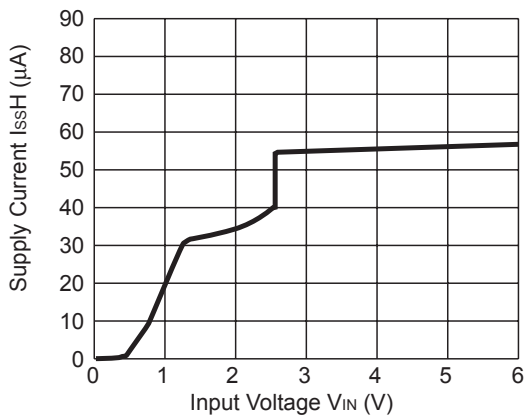
R1161x26xx (ECO=H)
