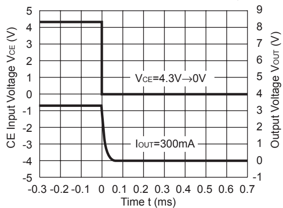
R1161x33xD
