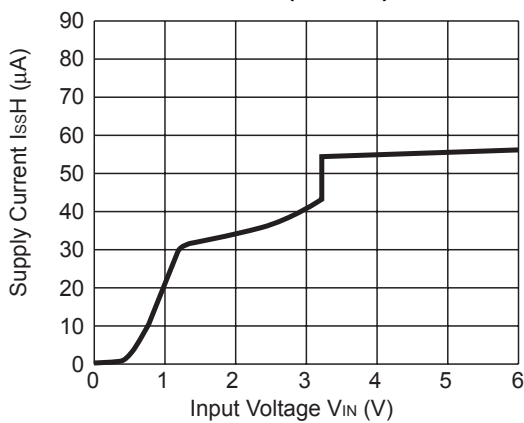
R1161x33xx (ECO=H)
