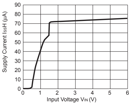
R1161x15xx (ECO=H)
