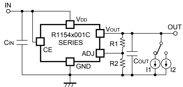
R1154x001C Load Transient Response Test Circuit
