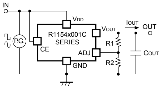
R1154x001C Input Transient Response Test Circuit
