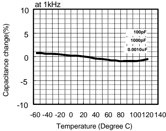
Temperature Characteristics
