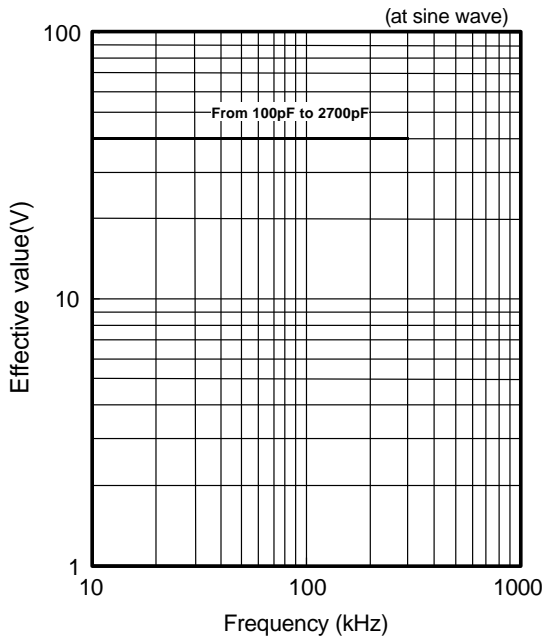
Permissible Voltage
