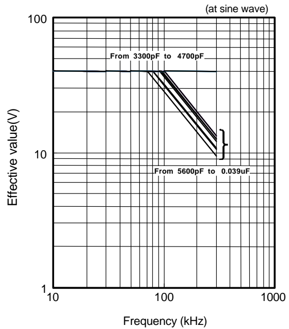
Permissible Voltage
