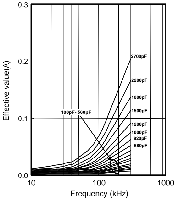
Permissible Current
