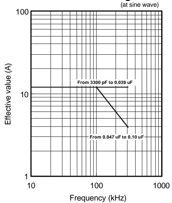
Permissible Voltage
