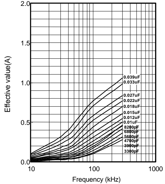
Permissible Current
