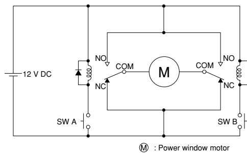
(M) : Power window motor
