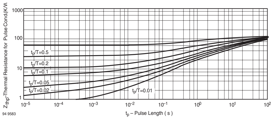
Figure 5. Thermal Response
