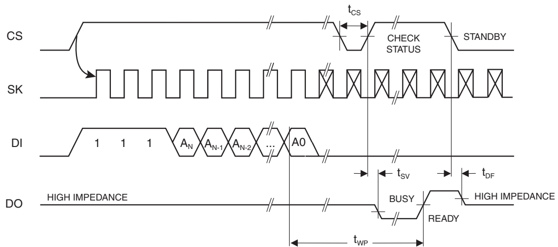
Figure 5-7. ERASE Timing
