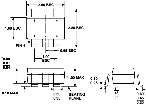
Figure 65. 5-Lead Thin Small Outline Transistor Package [TSOT] (UJ-5)
