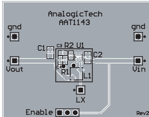
Figure 2: AAT1143 Evaluation Board Top Side.
