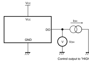
Fig.4 "HIGH" output voltage circuit
