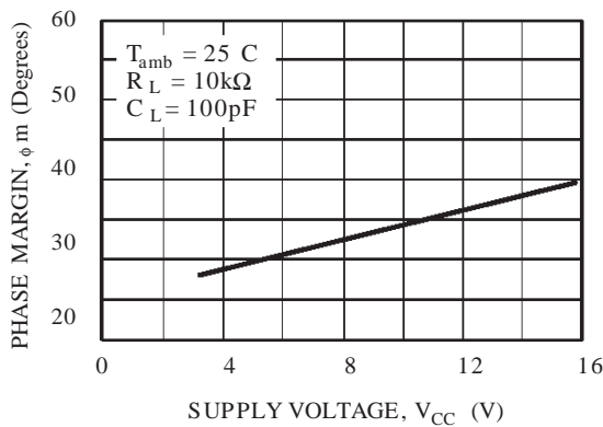
Figure 7a : Phase Margin vs Supply Voltage
