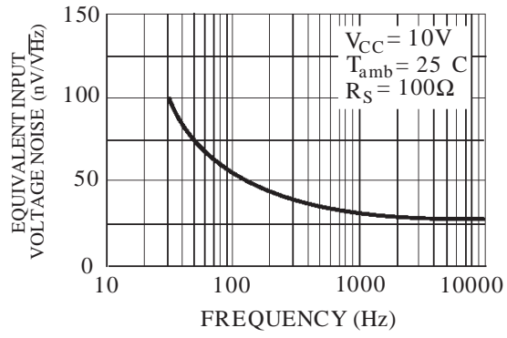
Figure 8 : Input Voltage Noise vs Frequency
