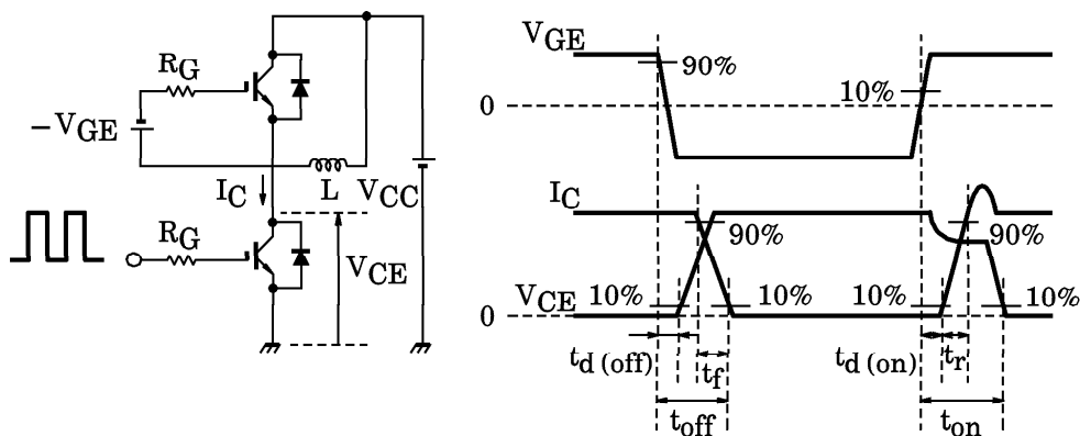
Note 1 Switching Time Test Circuit & Timing Chert
