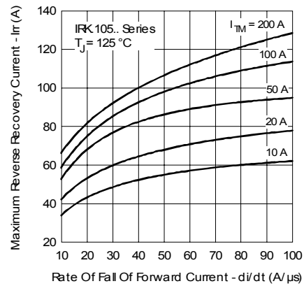
Fig. 12 - Recovery Current Characteristics
