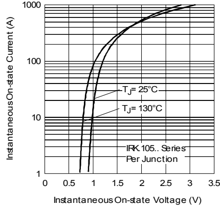
Fig. 10 - On-state Voltage Drop Characteristics
