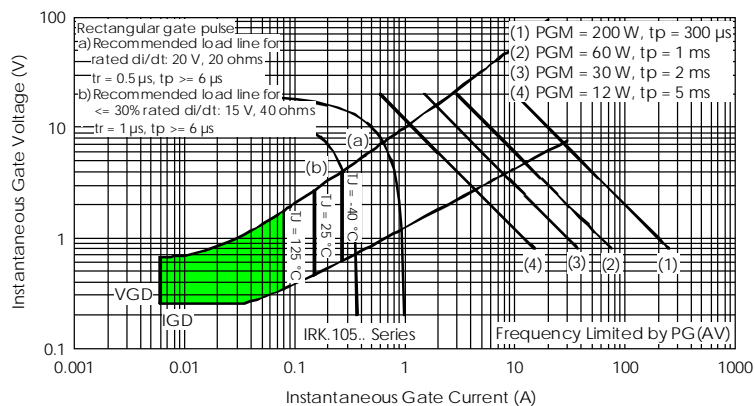
Fig. 14- Gate Characteristics
