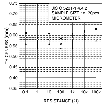
Fig.4 Dimensions (thickness)
