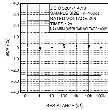
Fig.7 Overload
