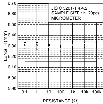
Fig.2 Dimensions (length)
