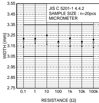
Fig.3 Dimensions (width)
