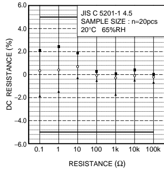
Fig.5 Resistance
