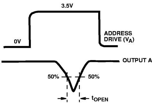
FIGURE 9B. WAVEFORMS
