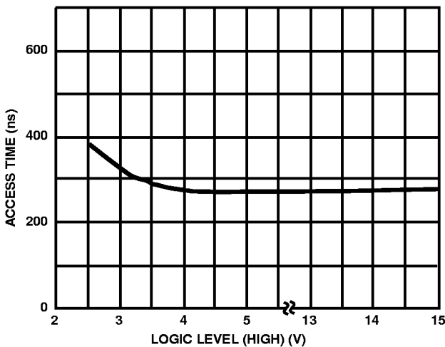
FIGURE 8A. ACCESS TIME vs LOGIC LEVEL (HIGH)
