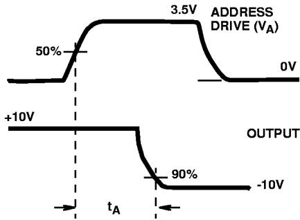
FIGURE 8C. WAVEFORMS
