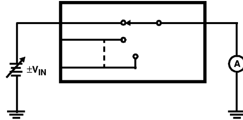
FIGURE 6B. TEST CIRCUIT
