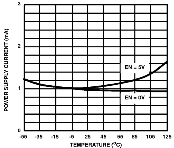
FIGURE 5B. HI-508/HI-509
