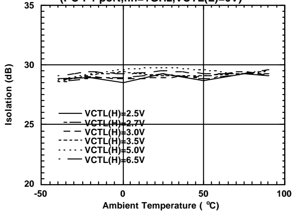
Isolation vs. Ambient Temperature (PC-P1 \text{ port}, f_{in}=1GHz, V_{CTL(L)}=0V)
