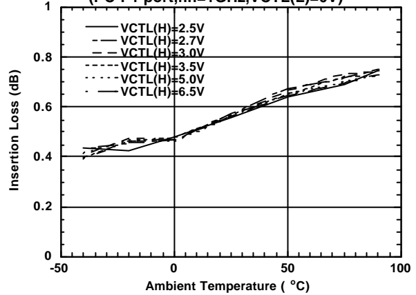
Insertion Loss vs. Ambient Temperature (PC-P1 \text{ port}, f_{in}=1GHz, V_{CTL(L)}=0V)
