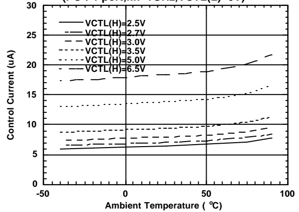
ICTL vs. Ambient Temperature (PC-P1 \text{ port}, f_{in}=1GHz, V_{CTL(L)}=0V)
