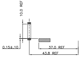
SECTION A-A FROM BEZEL TO [K] & [L]
