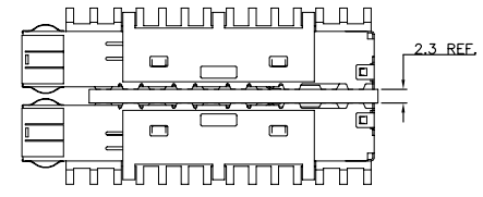
BEZEL CUTOUT LOCATIONS FOR BELLY TO BELLY APPLICATIONS ARE DEPENDENT ON PCB THICKNESS
