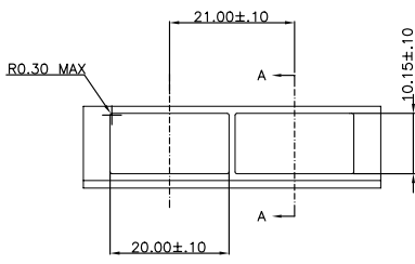
RECOMMENDED BEZEL DESIGN
