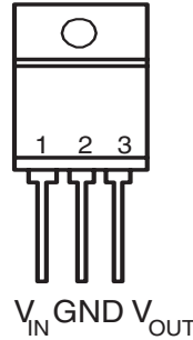
Front View TAB = GND
