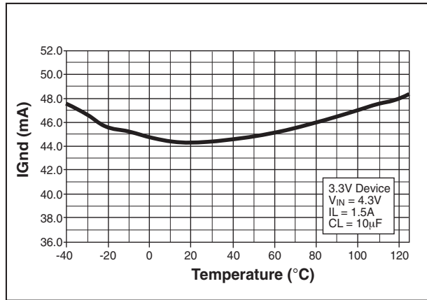
Figure 12. Ground Current vs Temperature at I_{LOAD} = 1.5A
