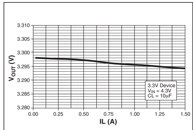
Figure 3. Load Regulation
