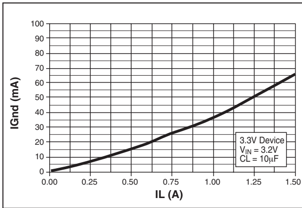
Figure 6. Ground Current vs Current in Dropout
