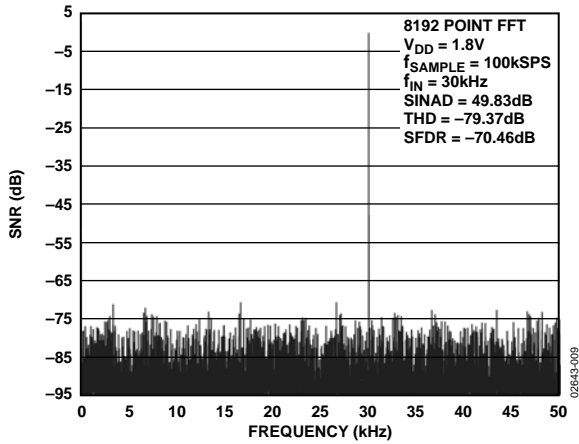
Figure 9. AD7468 Dynamic Performance at 100 kSPS
