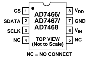
Figure 6. MSOP Pin Configuration
