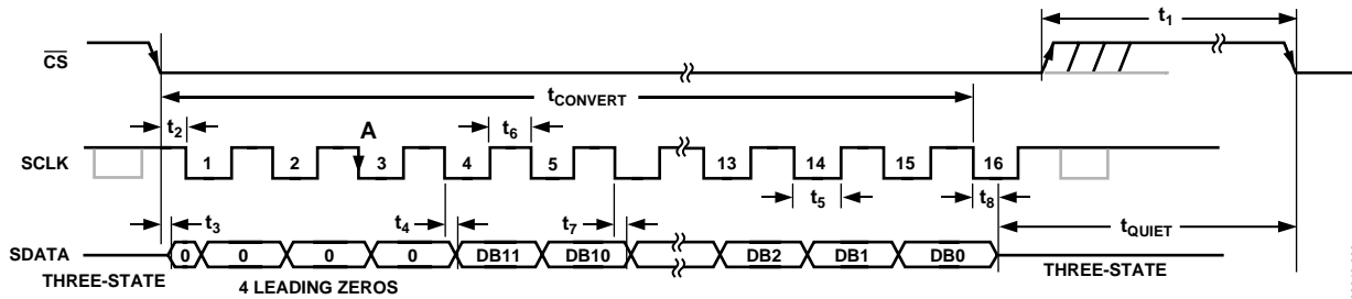
Figure 3. AD7466 Serial Interface Timing Diagram Example
