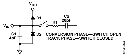
Figure 24. Equivalent Analog Input Circuit
