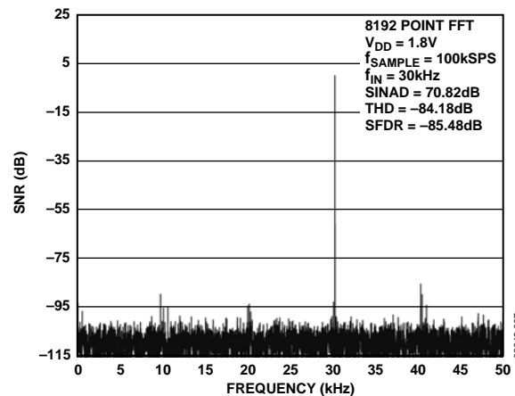
Figure 7. AD7466 Dynamic Performance at 100 kSPS
