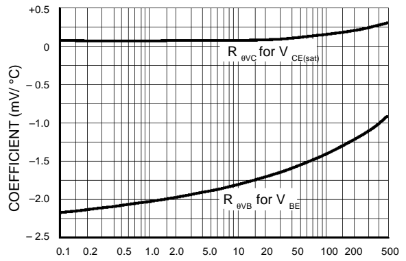
I_C , COLLECTOR CURRENT (mA) Figure 12. Temperature Coefficients
