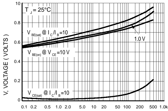
I_C , COLLECTOR CURRENT (mA) Figure 11. "On" Voltages
