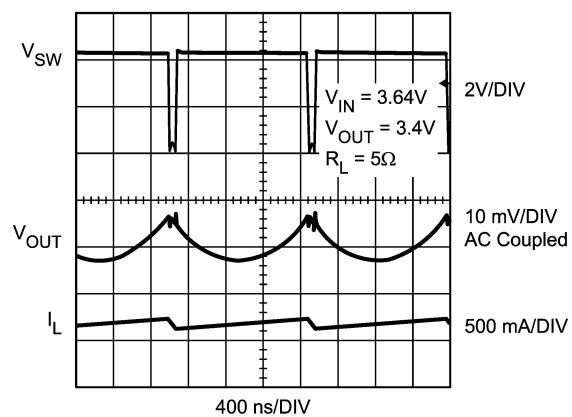
Output Voltage Ripple in Pulse Skip (V IN = 3.64V, V OUT = 3.4V, R LOAD = 5Ω)
