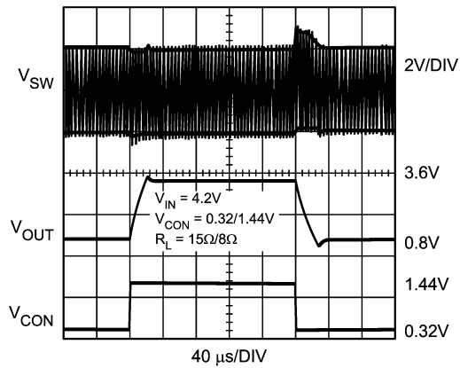
V CON and Load Transient (V IN = 4.2V, V CON = 0.32V/1.44V, R LOAD = 15Ω/8Ω)
