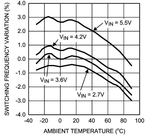
Switching Frequency vs Temperature ( V_{OUT} = 1.3V , I_{OUT} = 200mA )
