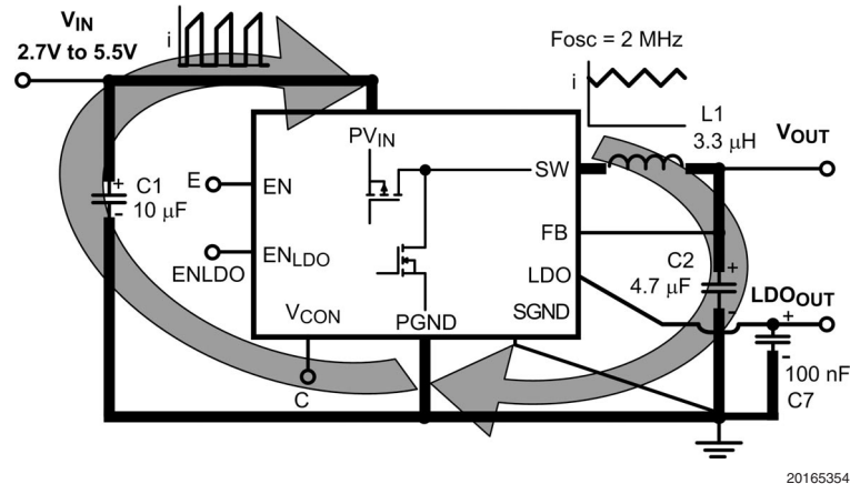
FIGURE 4. Current Loop
