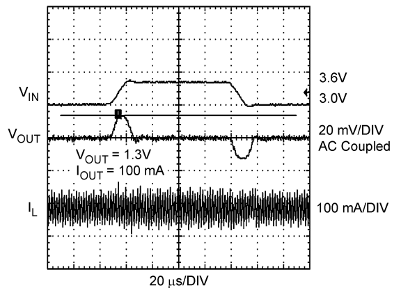
Line Transient Response ( V_{IN} = 3.0V \text{ to } 3.6V, I_{OUT} = 100mA )
