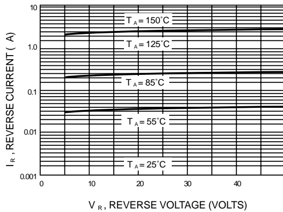
Figure 3. Leakage Current
