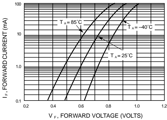
Figure 2. Forward Voltage
