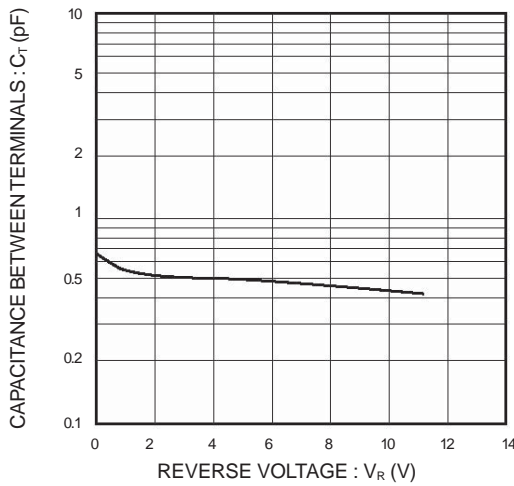
Fig.3 Capacitance between terminals
