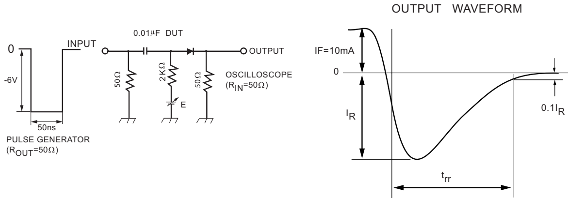
Fig.5 Reverse recovery time ( t_{rr} ) test circuit
