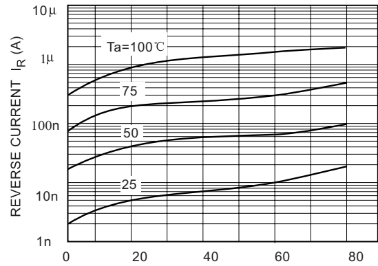
Fig.2 REVERSE VOLTAGE V_R (V)
