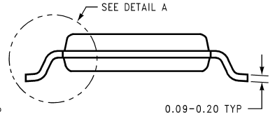
20-Lead Molded TSSOP, Exposed Pad, 6.5x4.4x0.9mm Order Number LM4863MTE NS Package Number MXA20A
