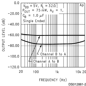
Channel Separation
