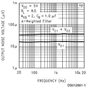
Noise Floor
