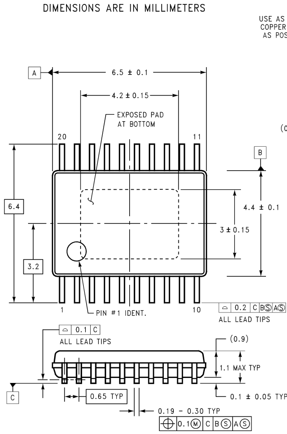
20-Lead Molded TSSOP, Exposed Pad, 6.5x4.4x0.9mm Order Number LM4863MTE NS Package Number MXA20A
