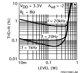
THD+N vs Output Power
