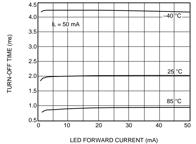
F. Turn-Off Time vs. LED Current (LH1504)
