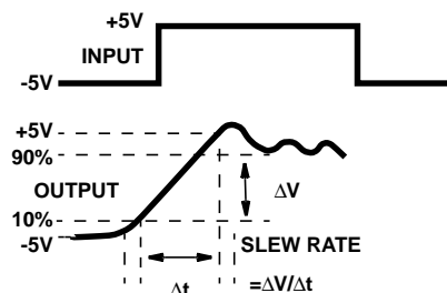
FIGURE 2. SLEW RATE
