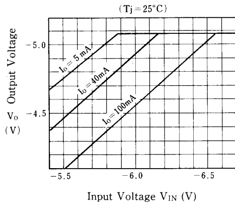
NJM79L05 Dropout Characteristics
