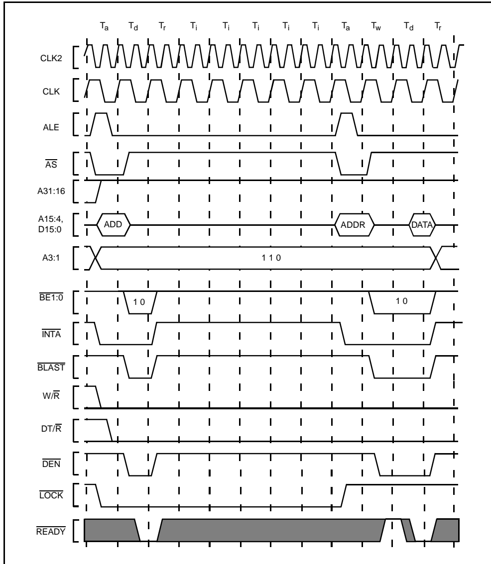
Figure 21. Interrupt Acknowledge Cycle
