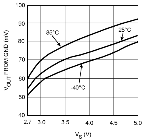
Output Negative Swing vs. Supply Voltage, R_L = 600\Omega
