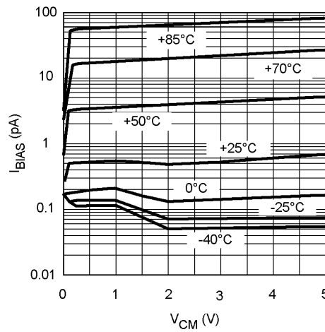
I_B vs. V_{CM} Over Temp
