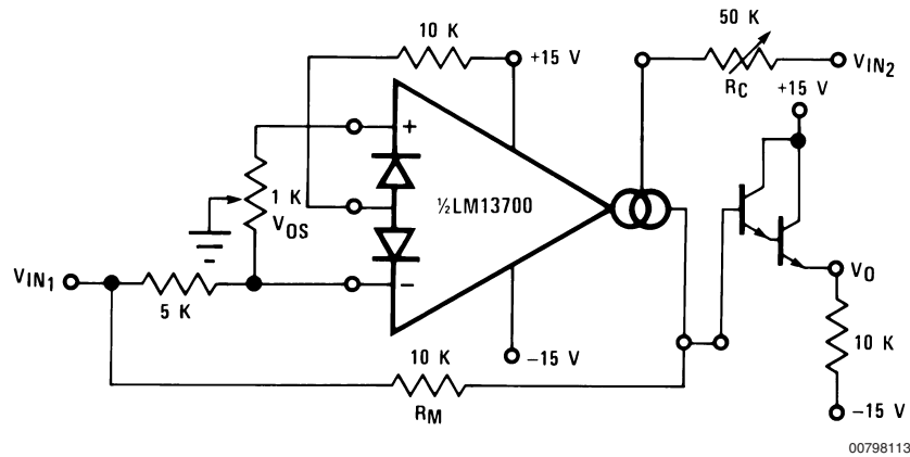
FIGURE 6. Four-Quadrant Multiplier
