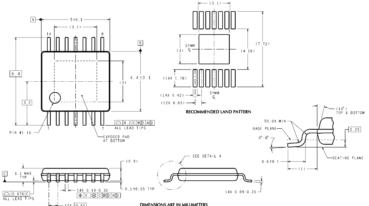
14-Lead Exposed Pad Plastic TSSOP Package NS Package Number MXA14A
