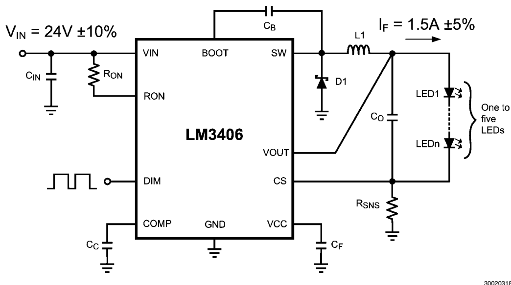
FIGURE 13. Schematic for Design Example 1
