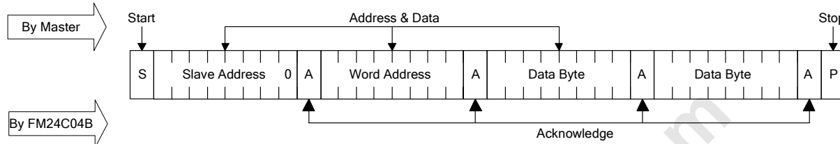
Figure 6. Multiple-Byte Write
