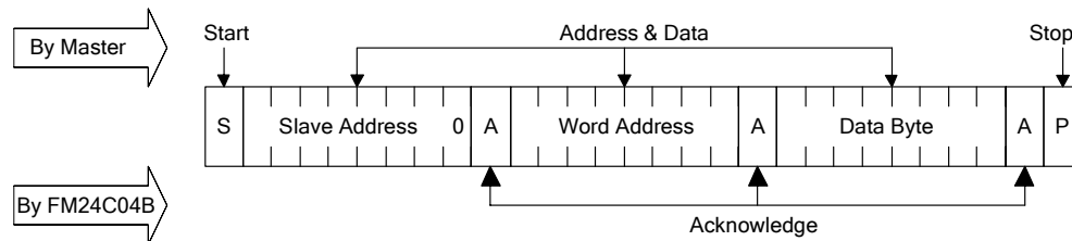
Figure 5. Byte Write
