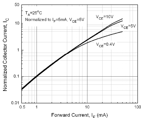
Figure 2. Normalized Collector Current vs Forward Current
