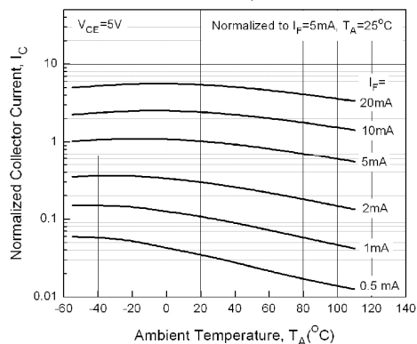
Figure 4. Normalized Collector Current vs Ambient Temperature
