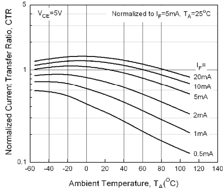
Figure 5. Normalized Current Transfer Ratio vs Ambient Temperature
