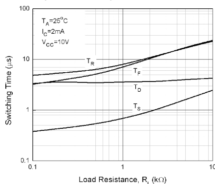
Figure 10. Switching Time vs Load Resistance
