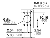
Recommended PC board pattern (BOTTOM VIEW)
