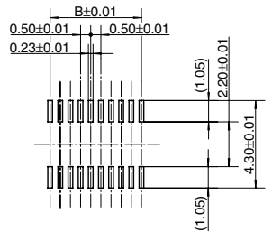
Recommended metal mask pattern Metal mask thickness: Here, 120 µm (Opening area ratio: 72%)
