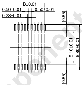
Recommended metal mask pattern Metal mask thickness: Here, 120 µm (Opening area ratio: 69%)
