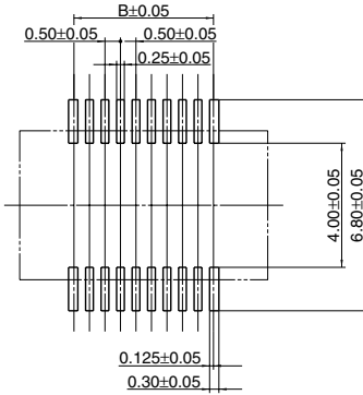
Recommended metal mask pattern Metal mask thickness: Here, 150 µm (Opening area ratio: 56%)
