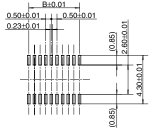
Recommended metal mask pattern Metal mask thickness: Here, 150 µm (Opening area ratio: 58%)
