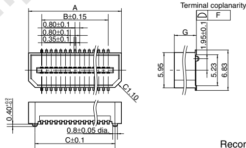
General tolerance: ±0.3
