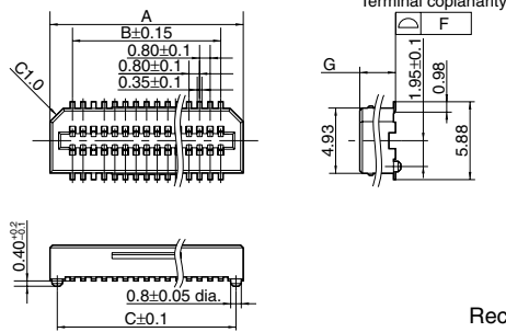
General tolerance: ±0.3
